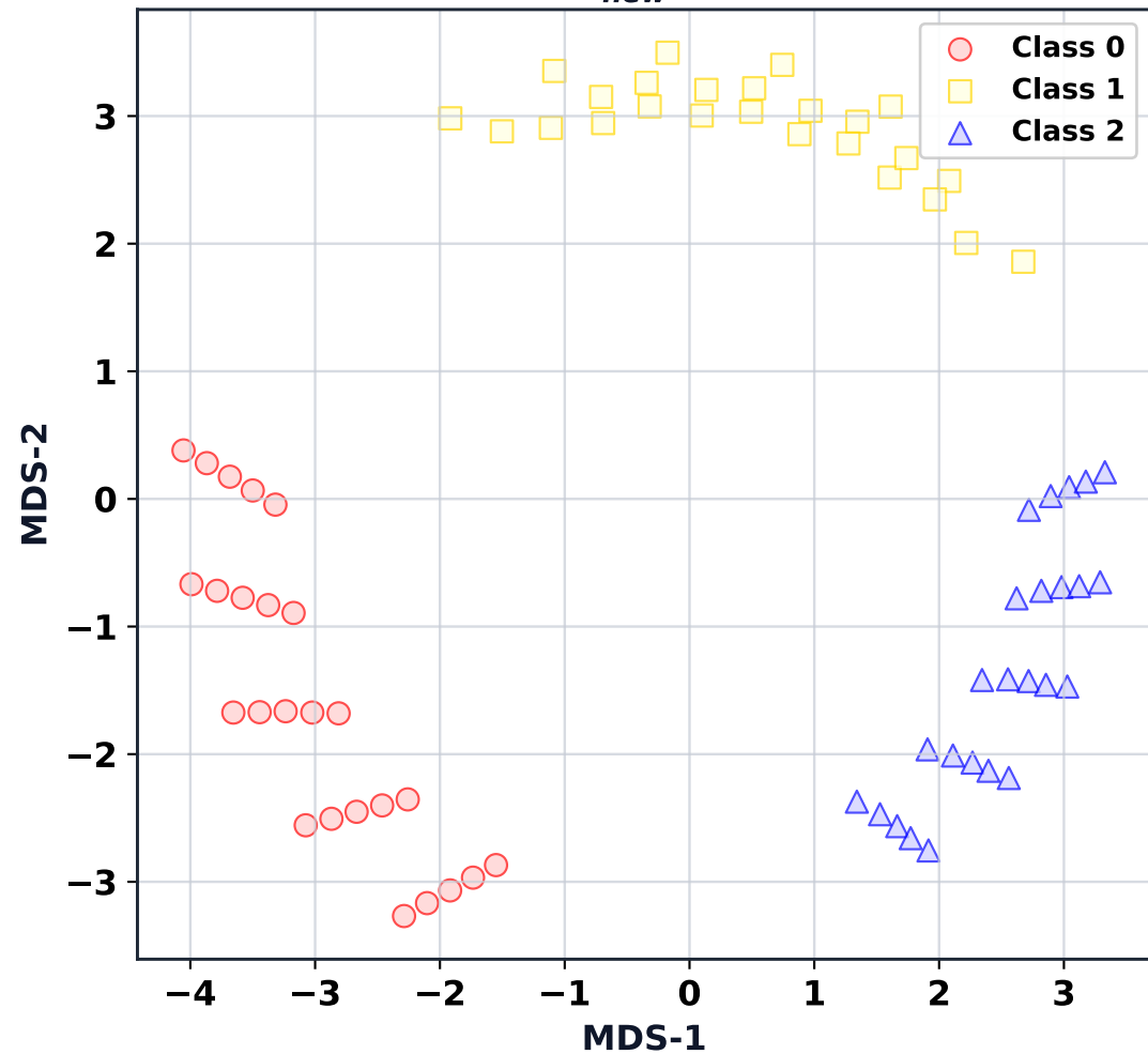
MDS: B_{new}^* (Order)
