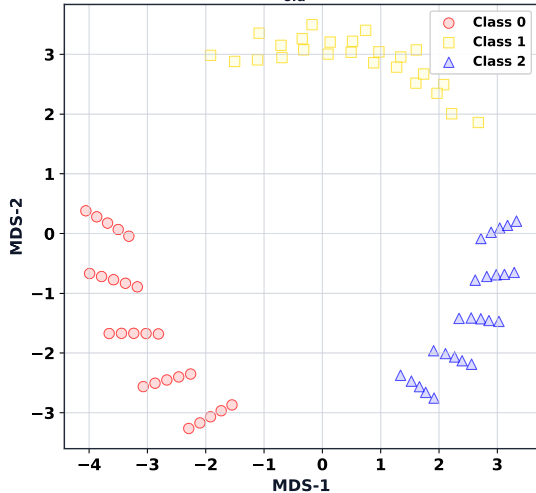
MDS: B_{old}^* (Chaos)
