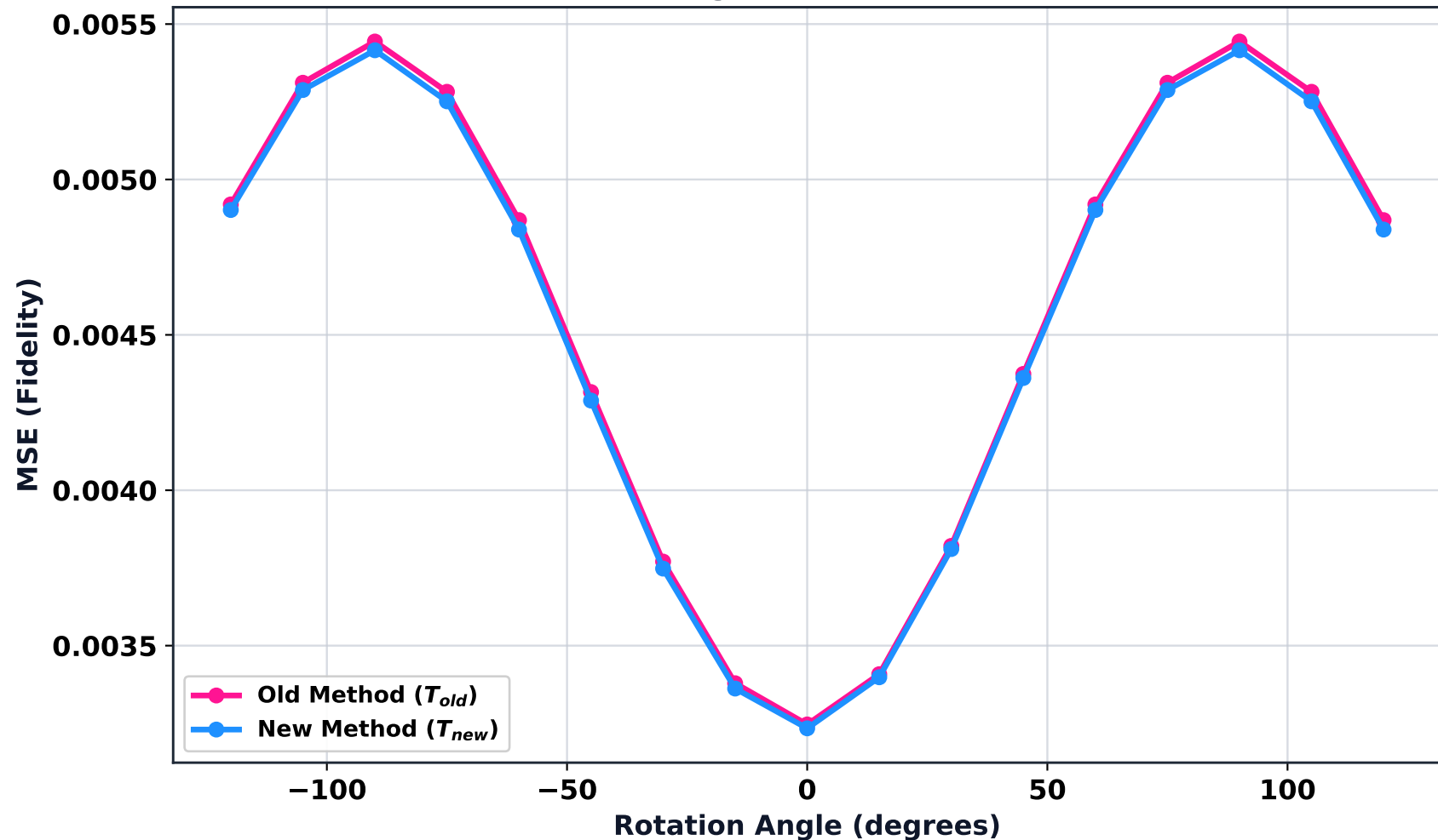
Robustness to Rotation (Stress Test) Range: [-120, 120]
