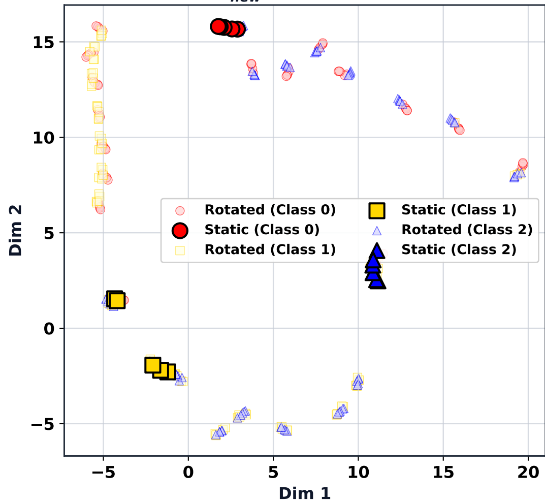
UMAP: B_{new}^* (Rotated vs Static)
