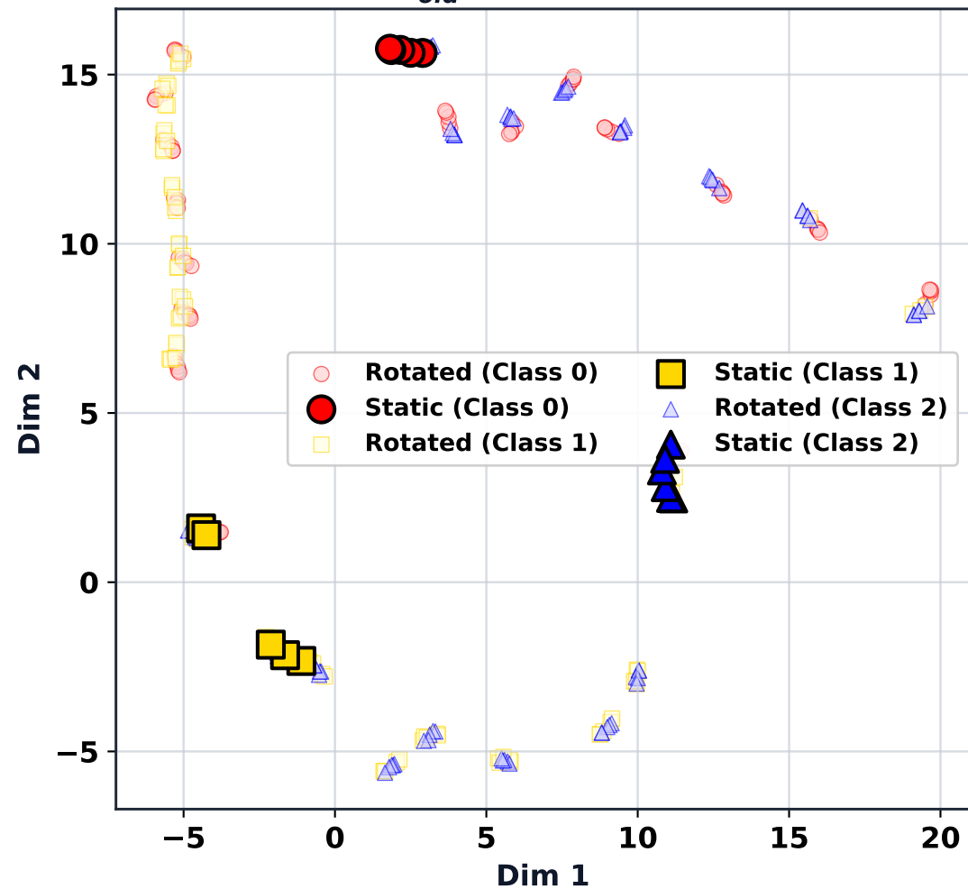
UMAP: B_{old}^* (Rotated vs Static)
