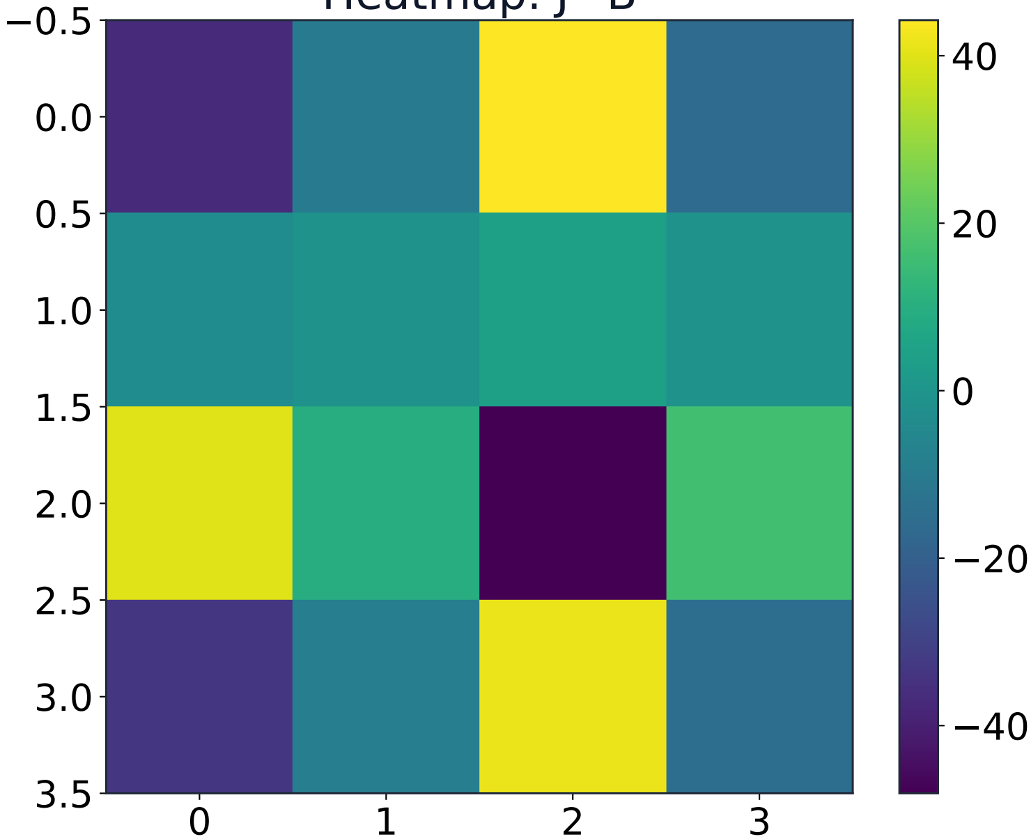
Heatmap: J^B
