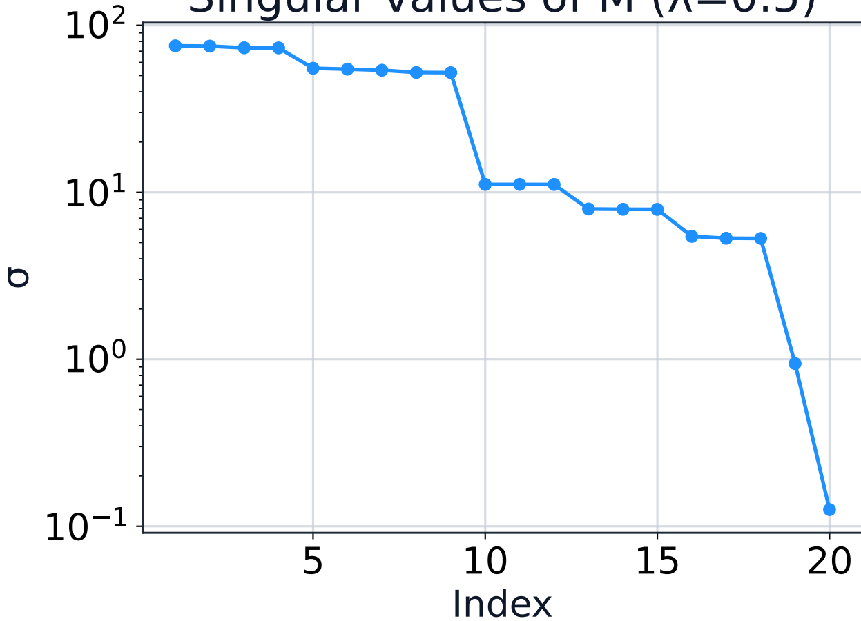
Singular values of M ( \lambda=0.5 )
