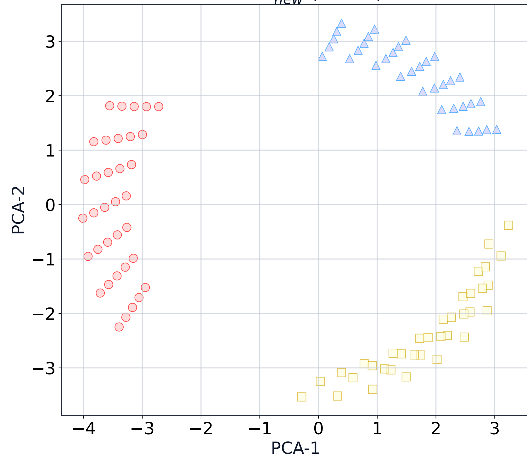
PCA: B_{new}^* (Order)
