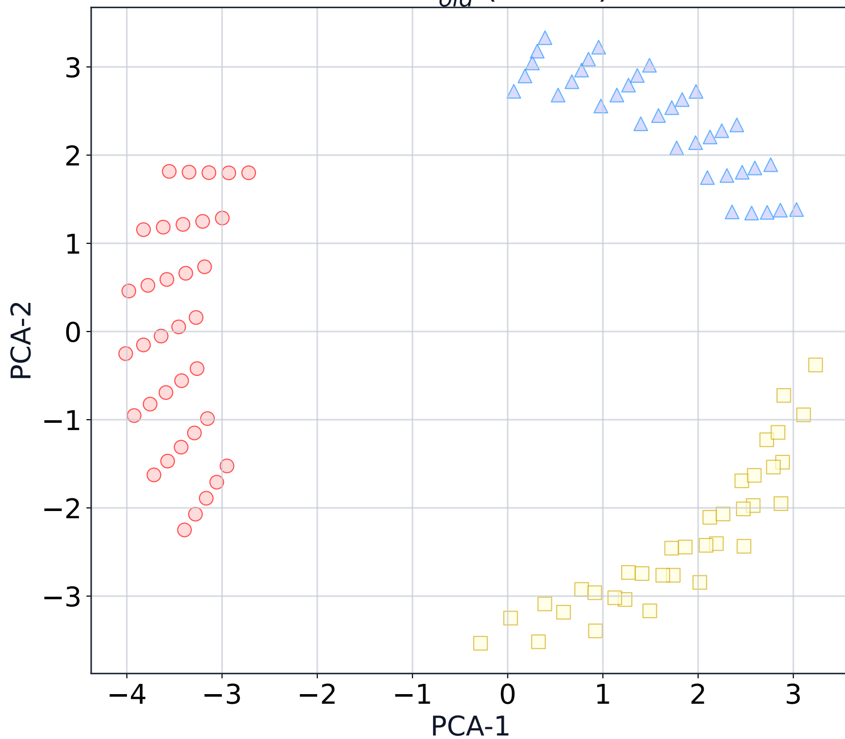
PCA: B_{old}^* (Chaos)
