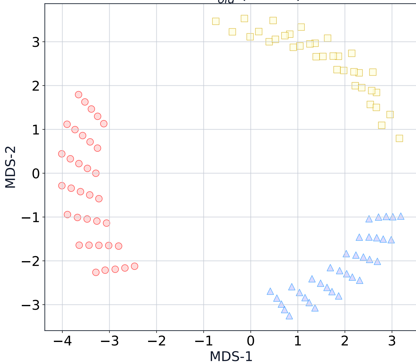
MDS: B_{old}^* (Chaos)
