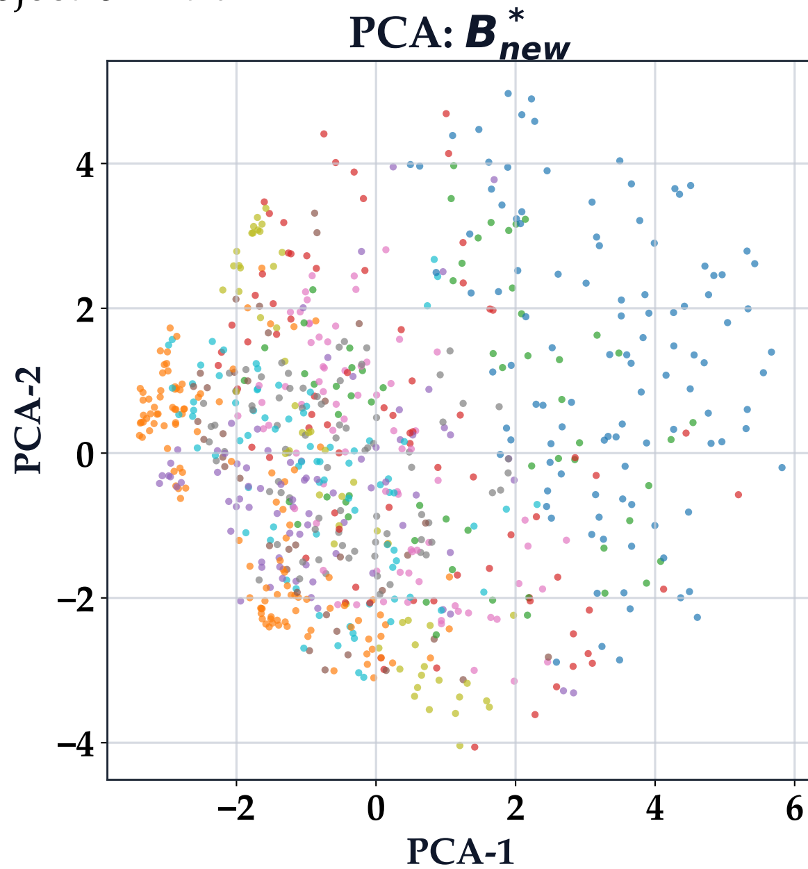
PCA Projection - train
