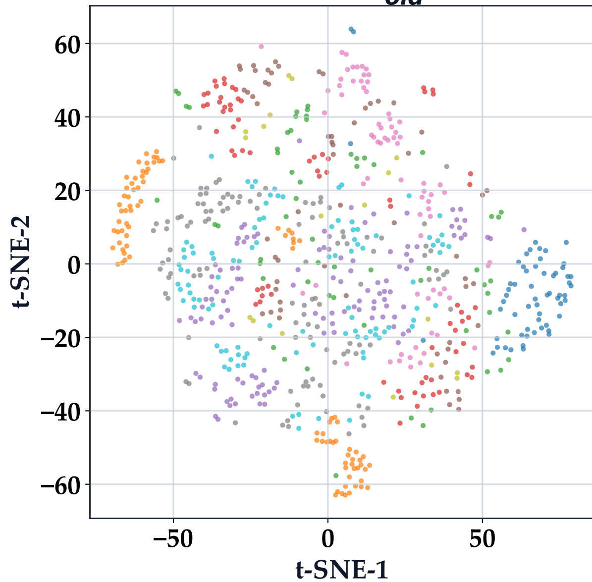
t-SNE: \mathbf{B}_{old}^*
