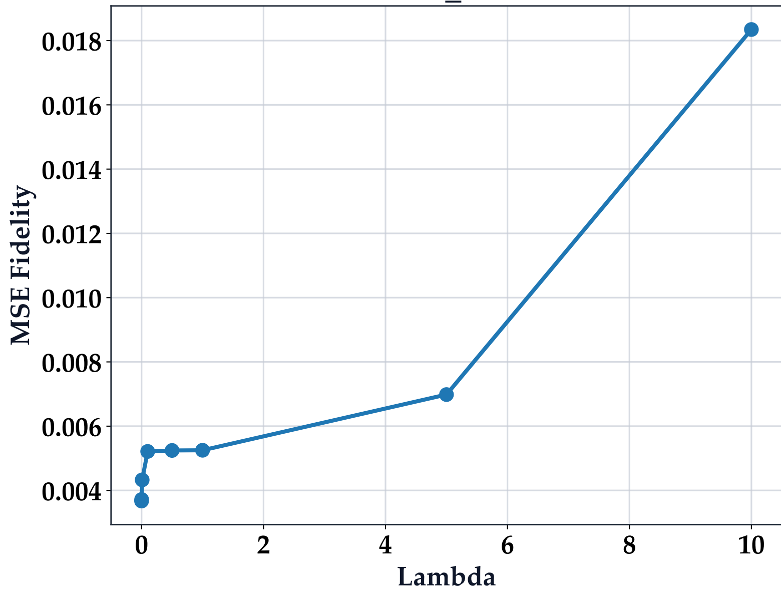
Trade-off: MSE_fid vs Lambda
