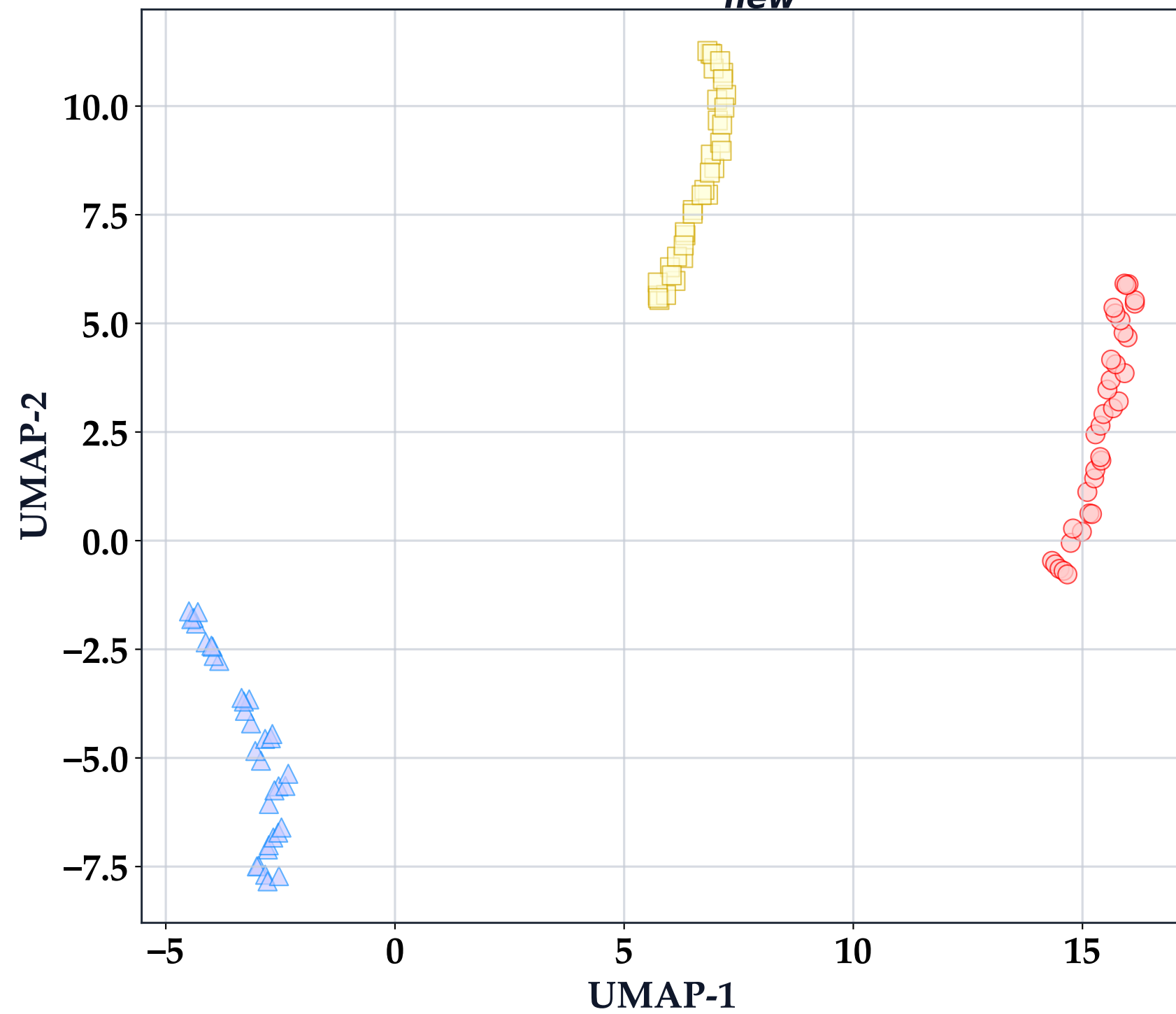
UMAP: B_{new}^*
