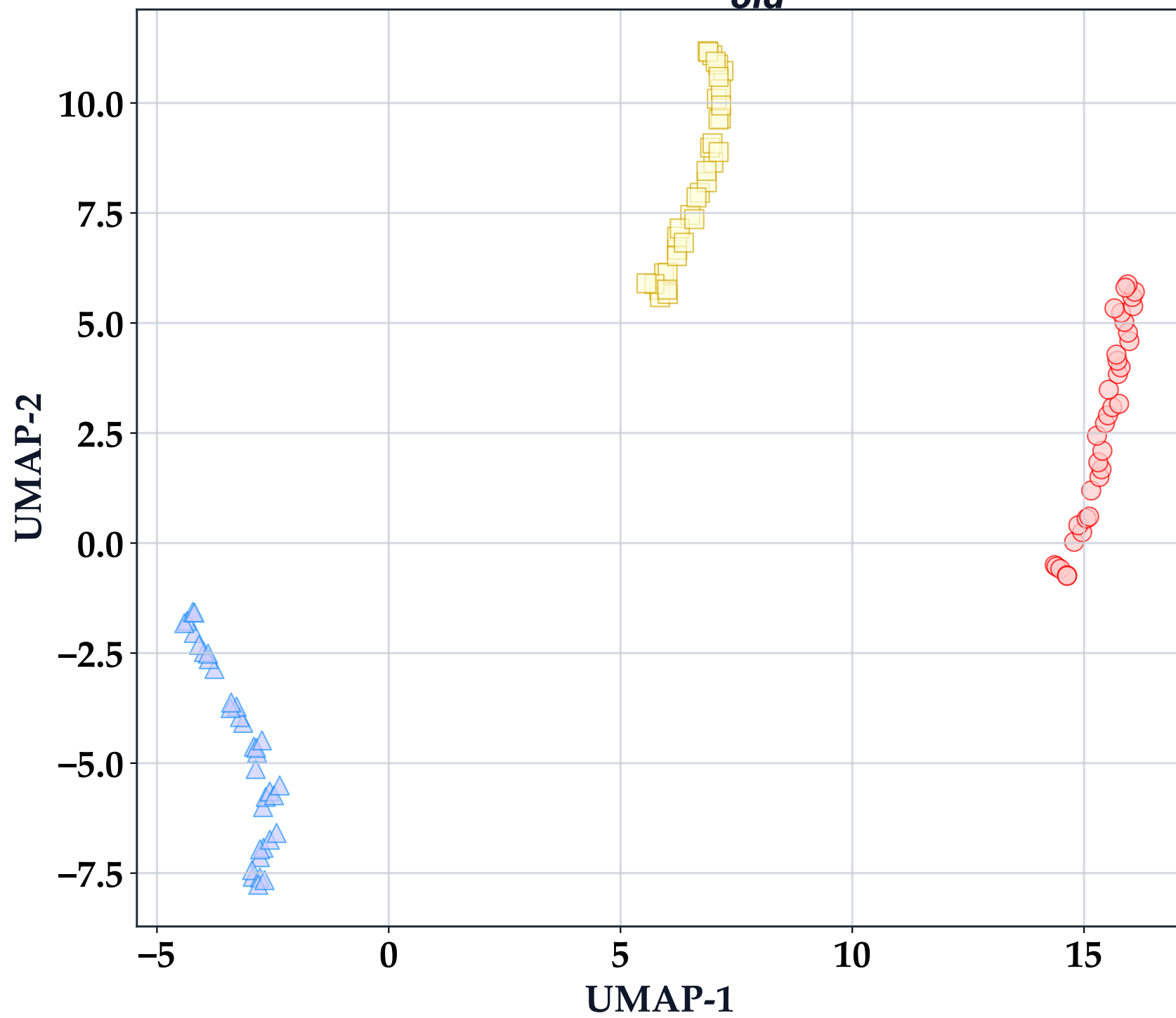
UMAP: B_{old}^*
