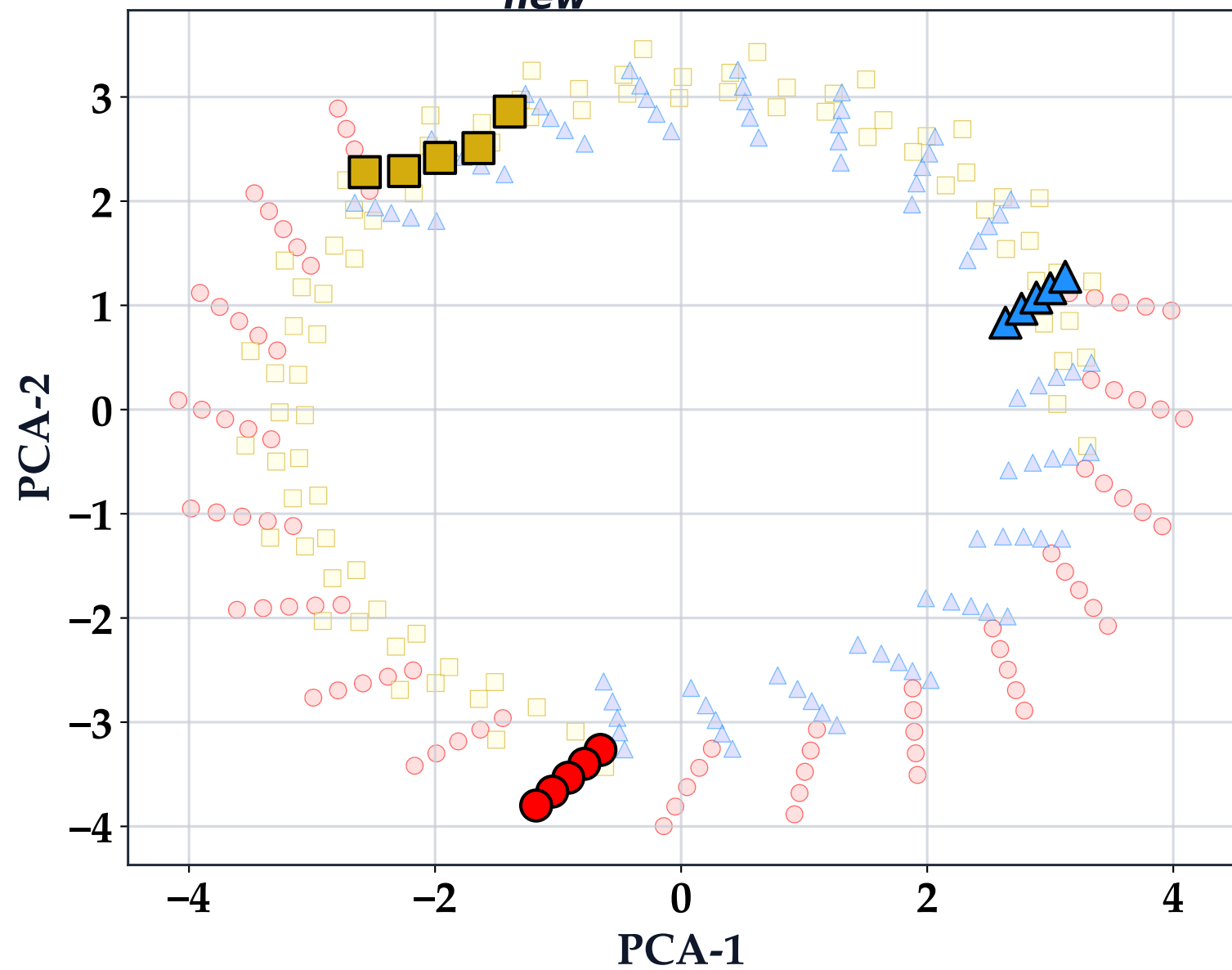
PCA: \mathbf{B}_{new}^* (Rotated vs Static)
