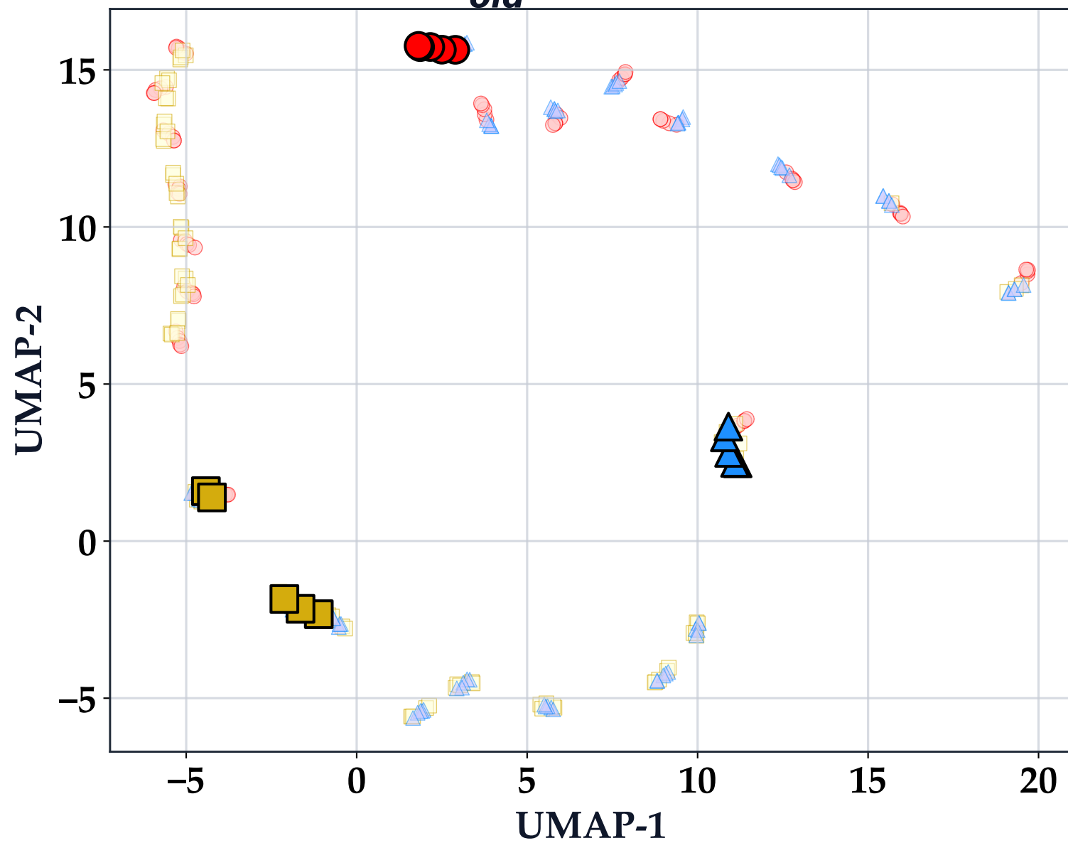
UMAP: \mathbf{B}_{old}^* (Rotated vs Static)
