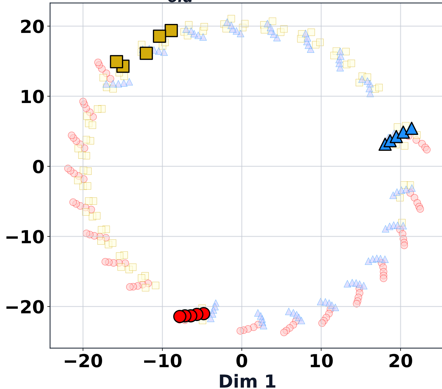
t-SNE: B_{old}^* (Rotated vs Static)
