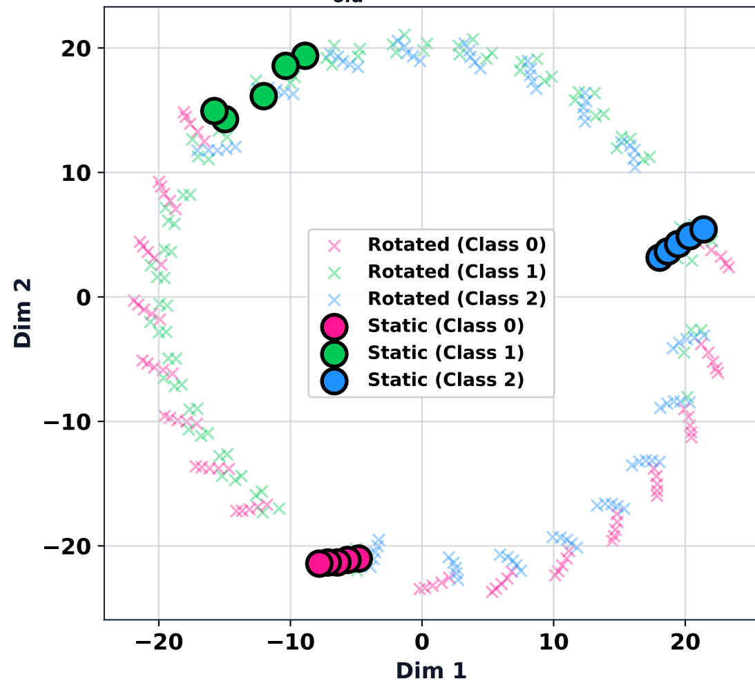
t-SNE: B_{old}^* (Rotated vs Static)
