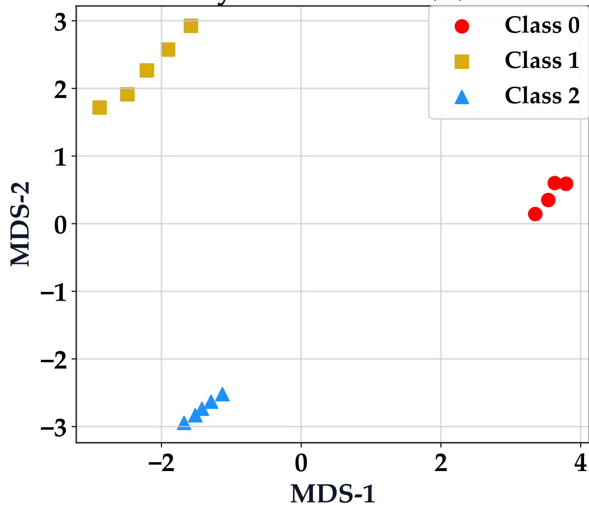
Synthetic: MDS(B)
