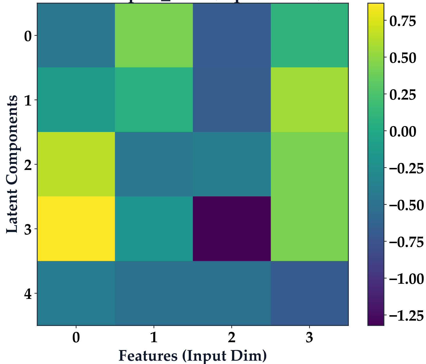
Heatmap: T_new (Equivariant)
