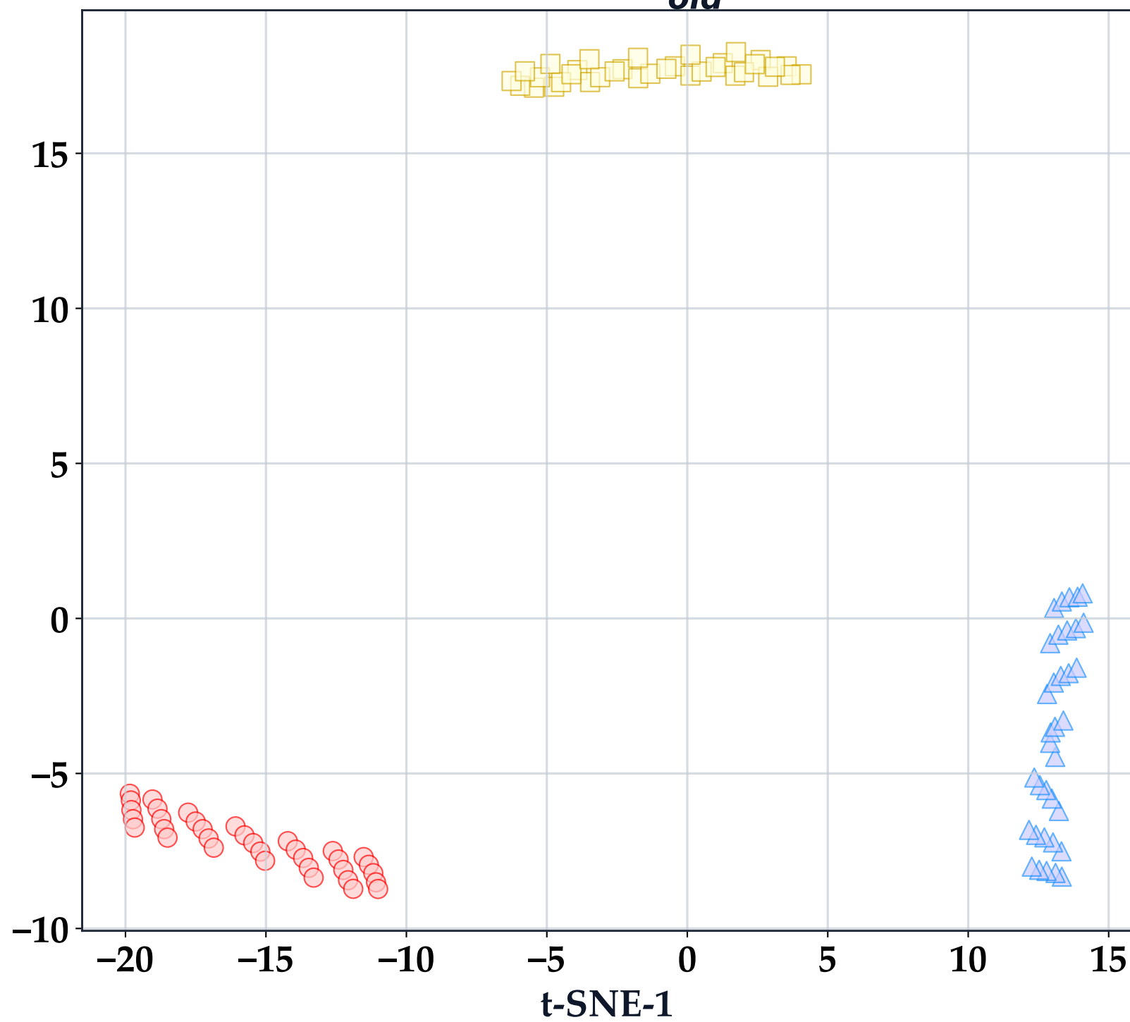
t-SNE: B_{old}^*
