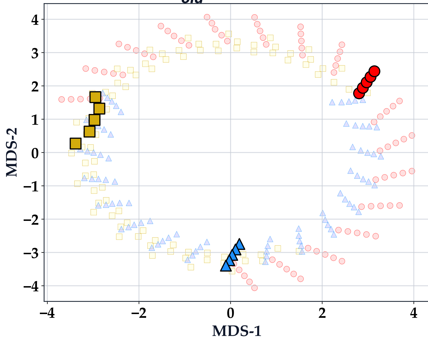
MDS: \mathbf{B}_{old}^* (Rotated vs Static)
