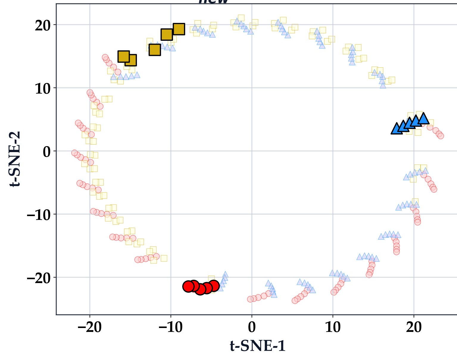
t-SNE: \mathbf{B}_{new}^* (Rotated vs Static)
