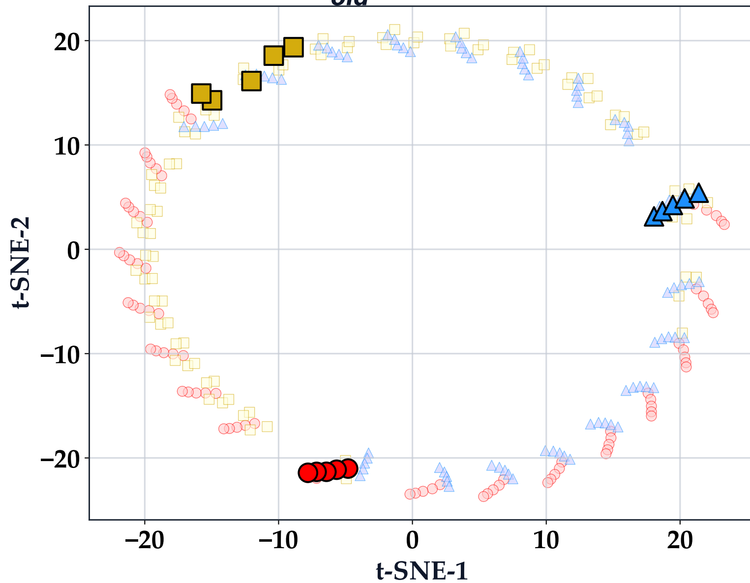
t-SNE: \mathbf{B}_{old}^* (Rotated vs Static)
