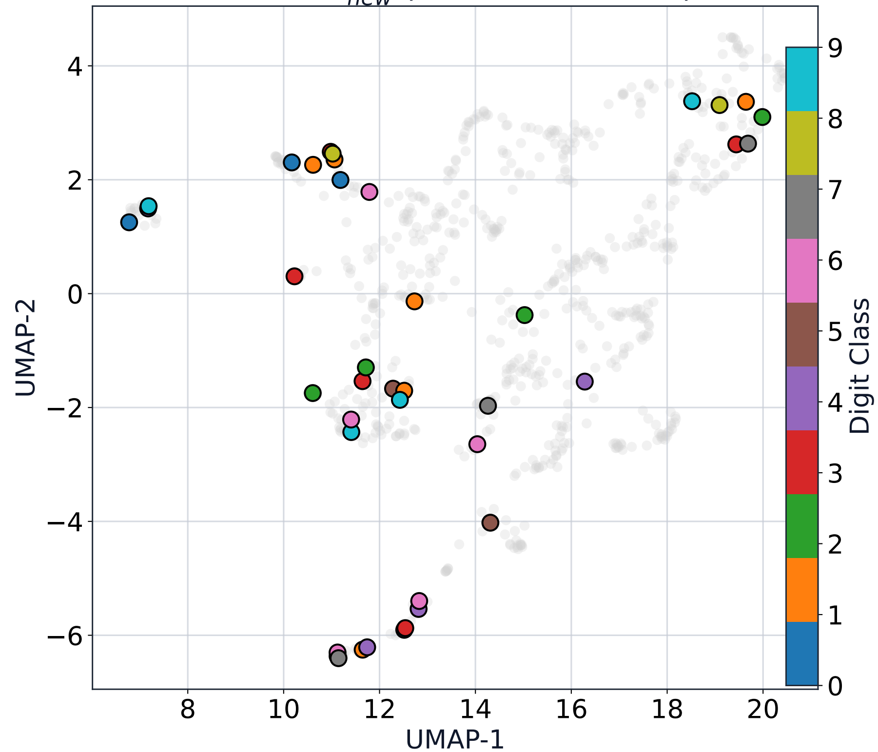
UMAP: B_{new}^* (Rotated vs Static)
