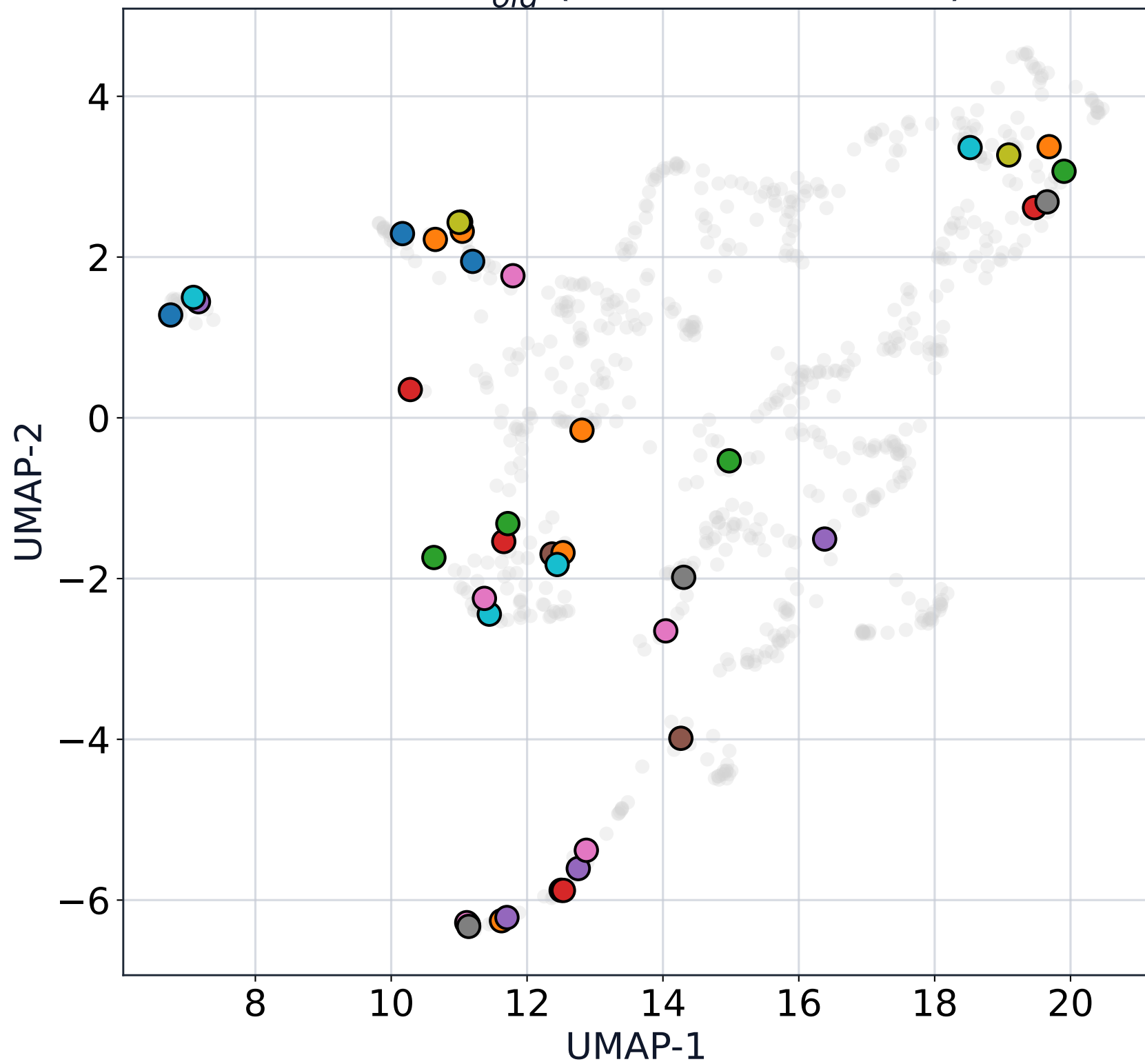
UMAP: B_{old}^* (Rotated vs Static)
