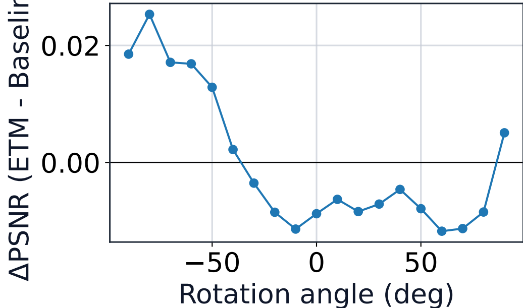
MNIST Robustness Gain: PSNR Difference vs Rotation
