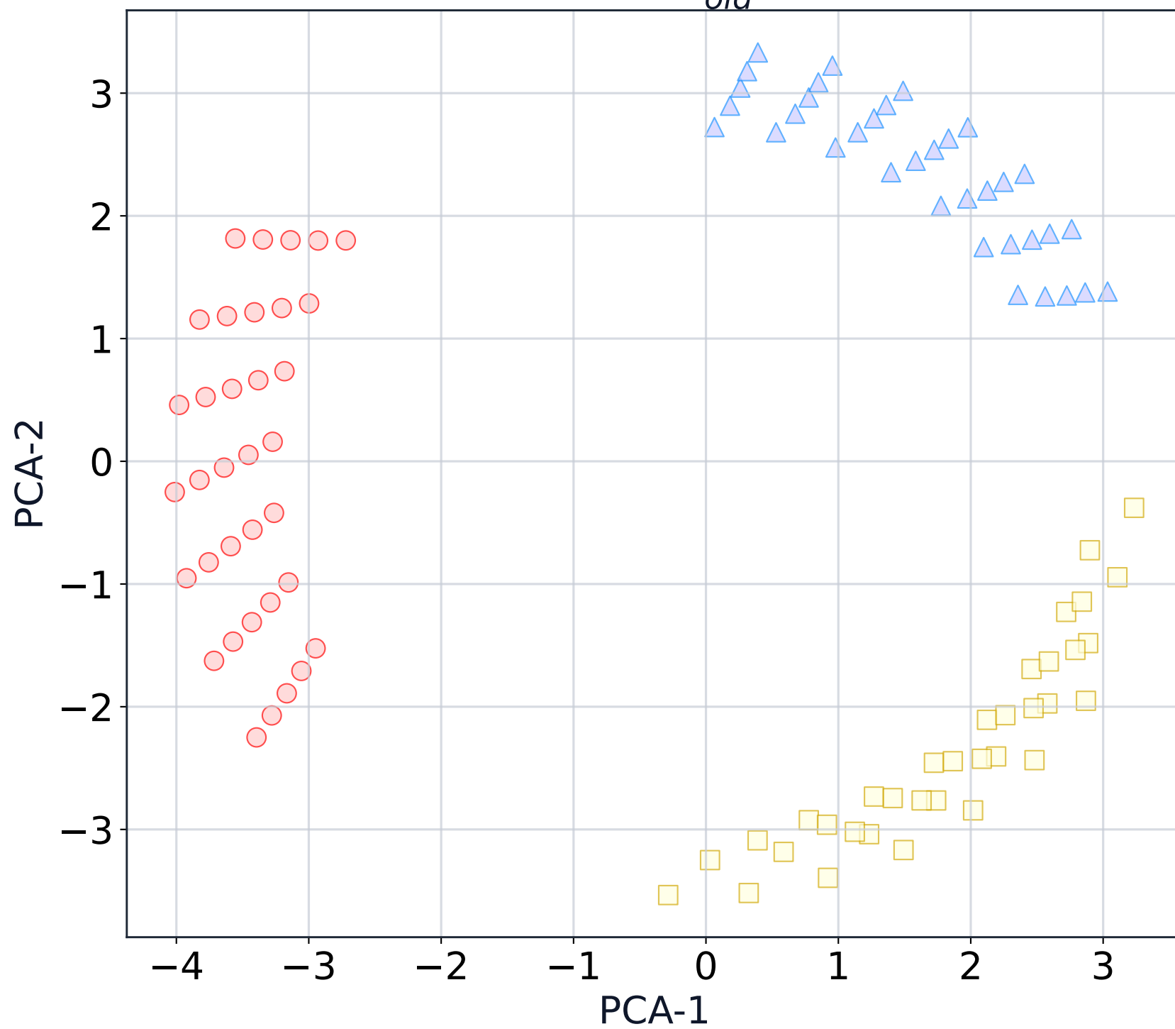
PCA: B_{old}^*
