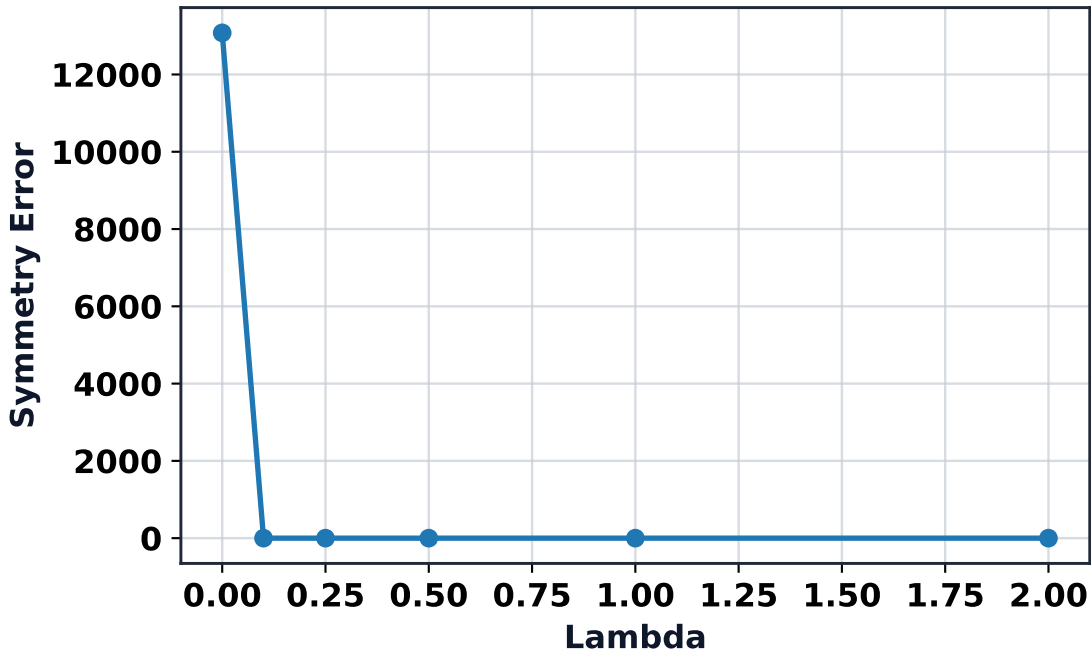
Trade-off: Symmetry Error vs Lambda
