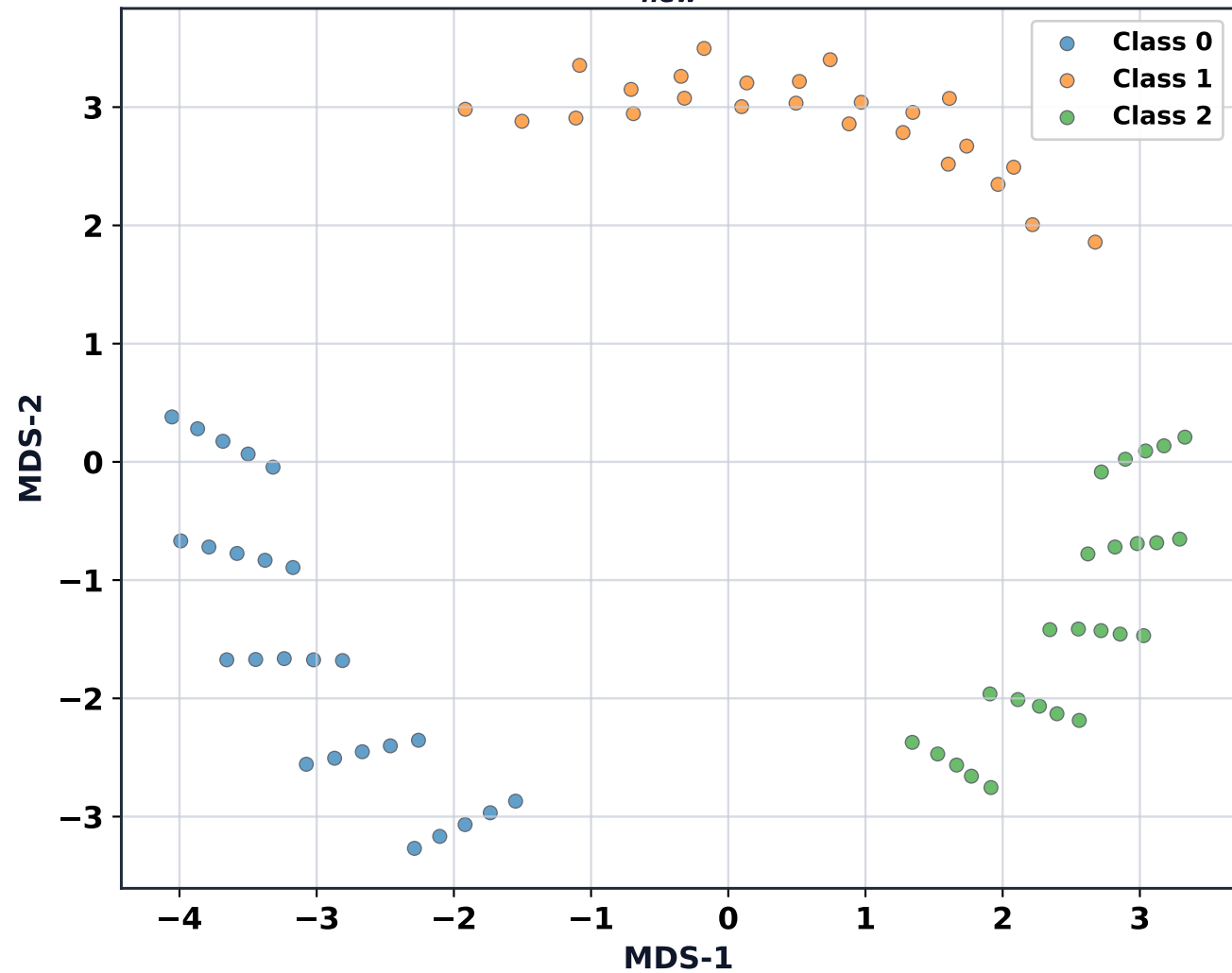
MDS: B_{new}^* (Order)
