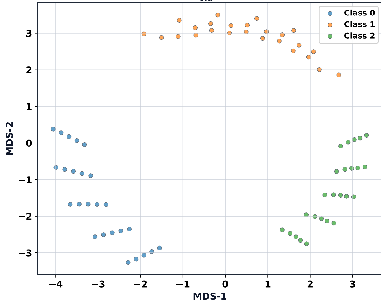
MDS: B_{old}^* (Chaos)
