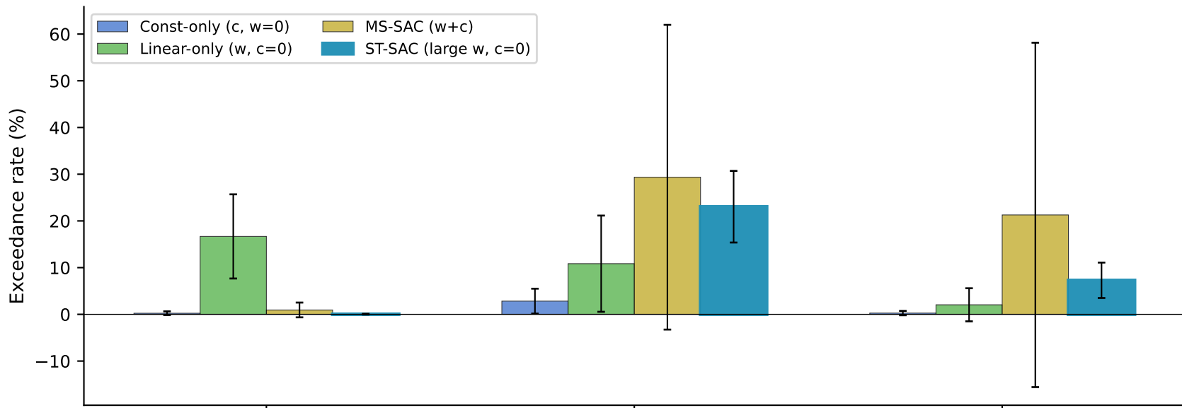
Reward component ablation — VR
