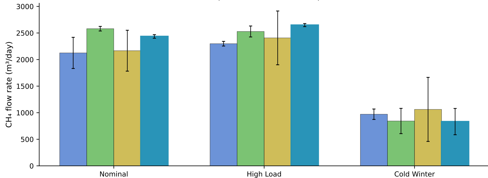
Reward component ablation — CH 4 production
