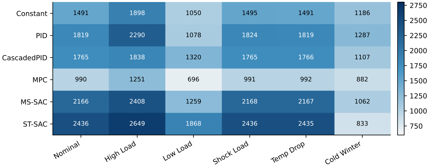
Average CH 4 flow rate (m 3 /day)
