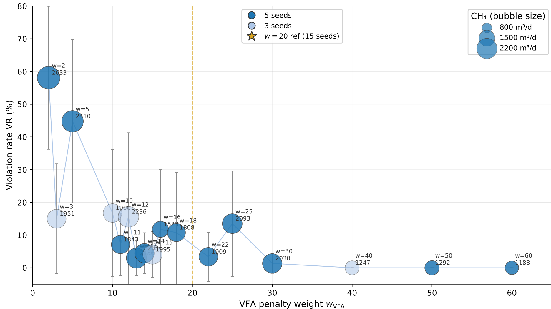
Nominal scenario: violation rate vs w_{\text{VFA}} (bubble size \propto CH 4 production)
