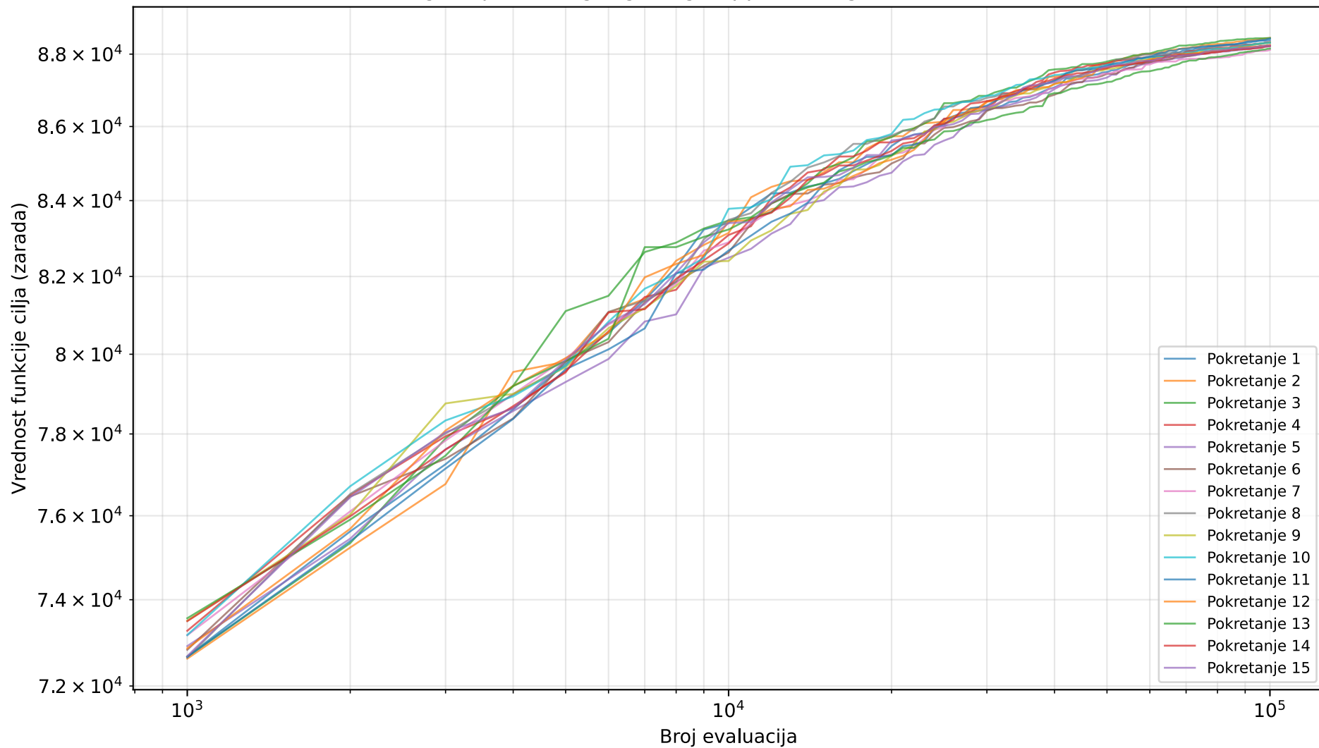
Konvergencija GA (log-log) — ga-cpp-convergence-1000-100-30.csv
