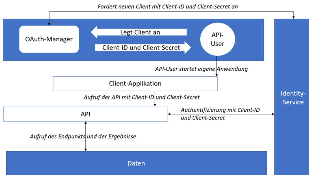
Abb.: OAuth-Client-Workflow
