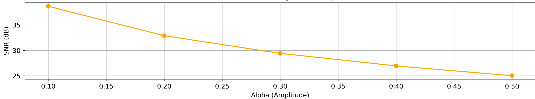
Spread Spectrum Watermarking: SNR vs Alpha
