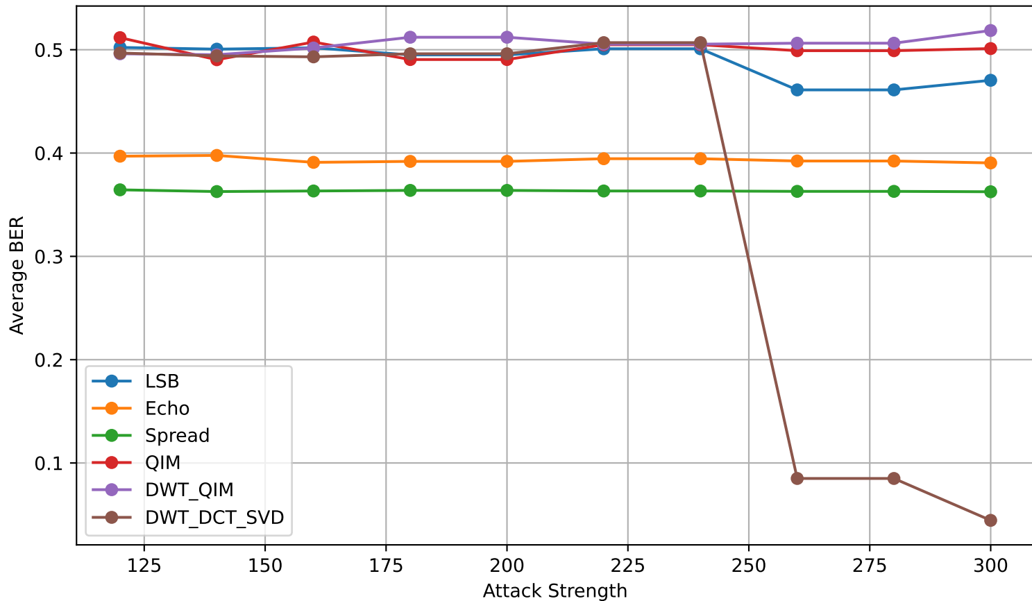
Robustness vs Attack Strength (compression)
