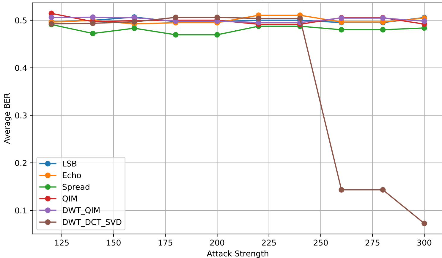
Robustness vs Attack Strength (compression)
