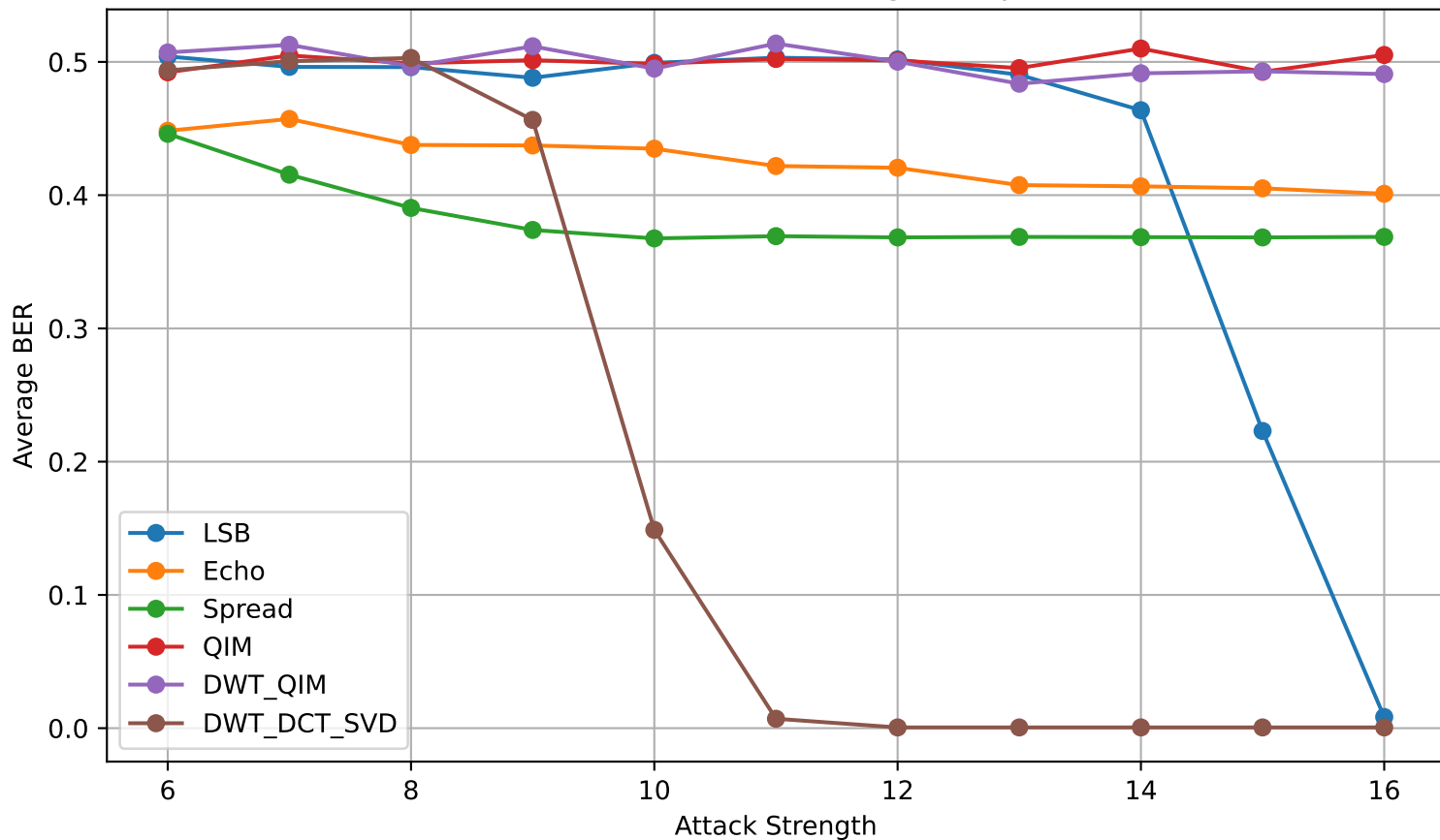
Robustness vs Attack Strength (requant)
