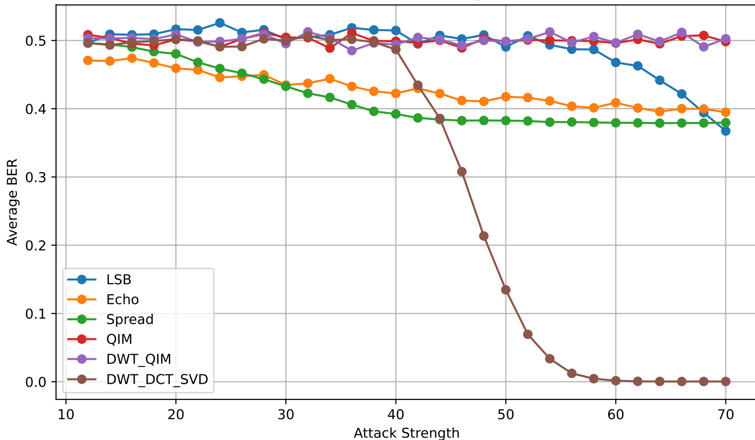
Robustness vs Attack Strength (noise)
