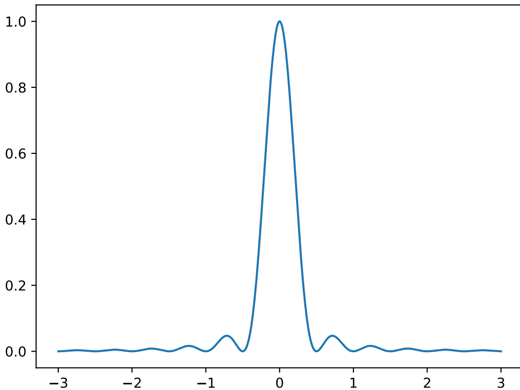
Sinc, B=2
