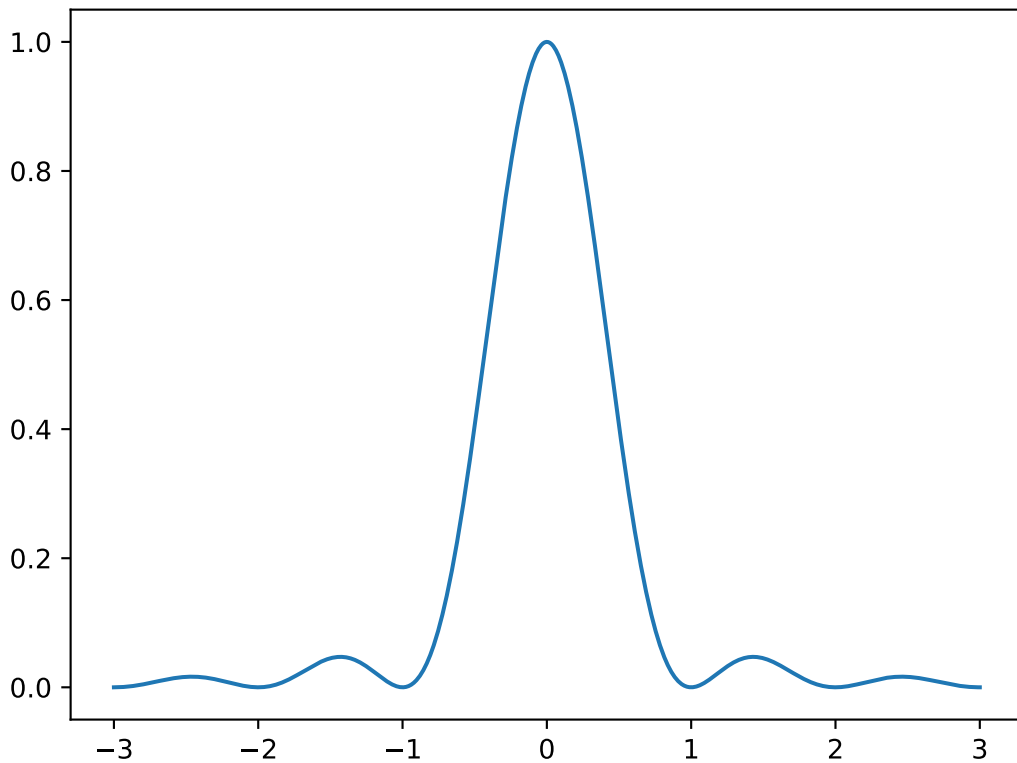
Sinc, B=1
