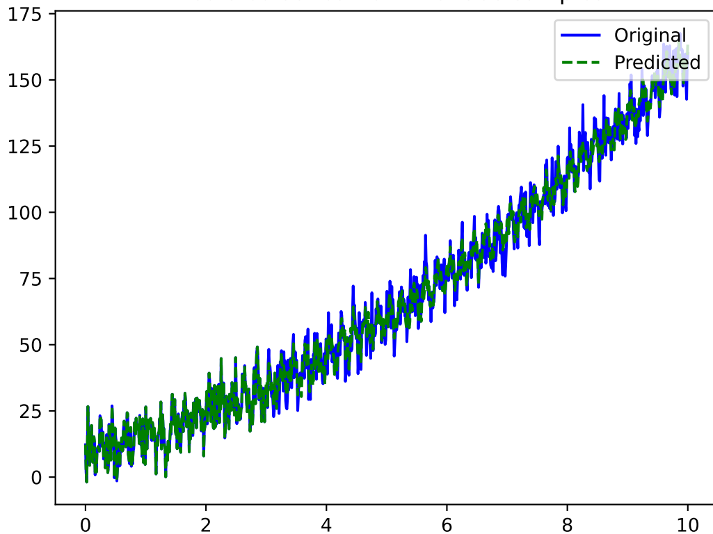
Predicted series from first 300 samples
