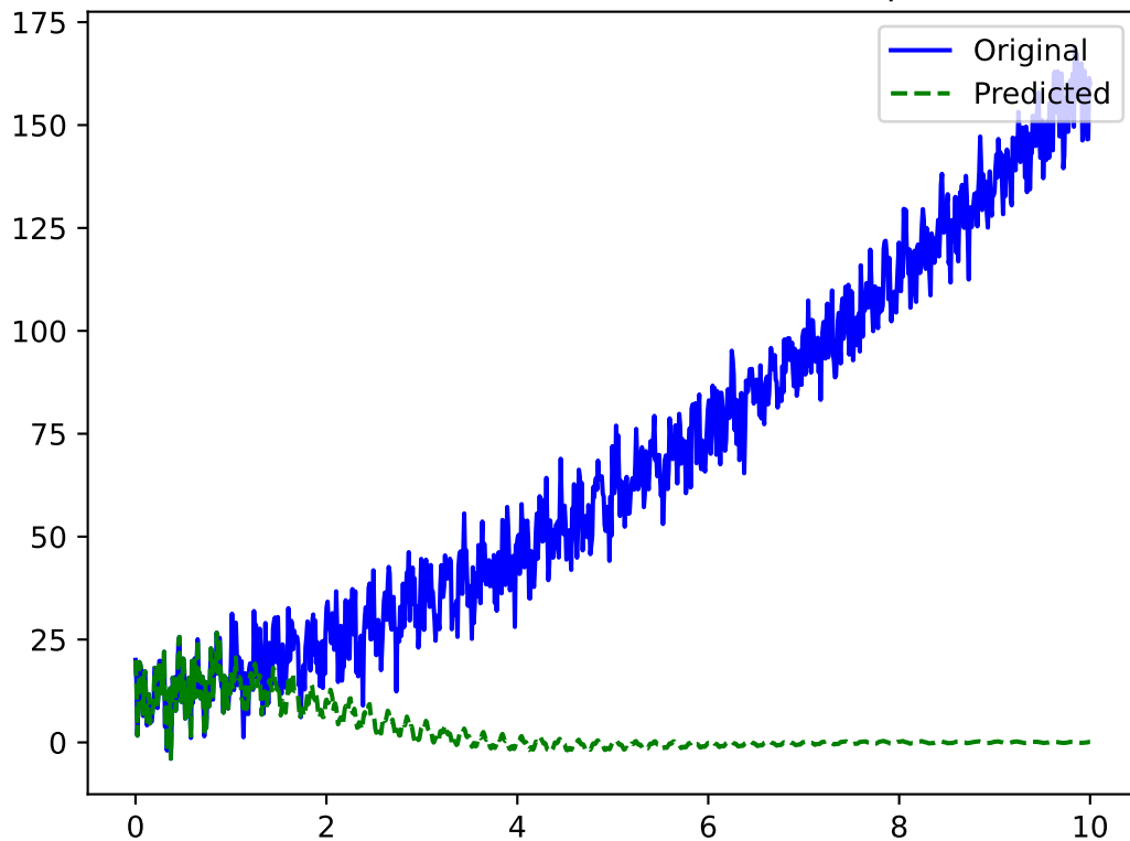
Predicted series from first 100 samples
