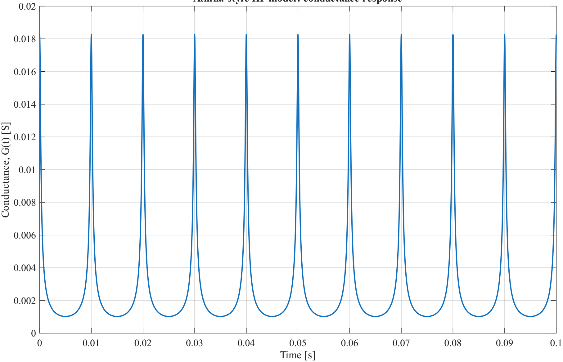
Athina-style HP model: conductance response
