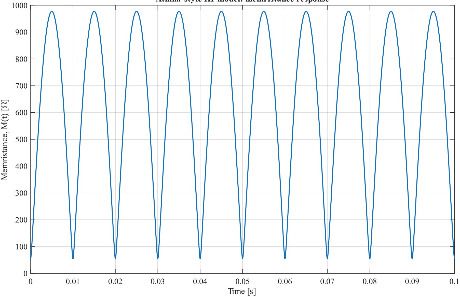
Athina-style HP model: memristance response
