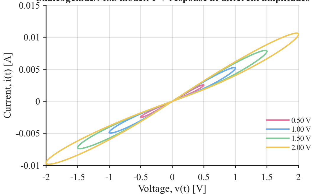
Chalcogenide/MSS model: I-V response at different amplitudes
