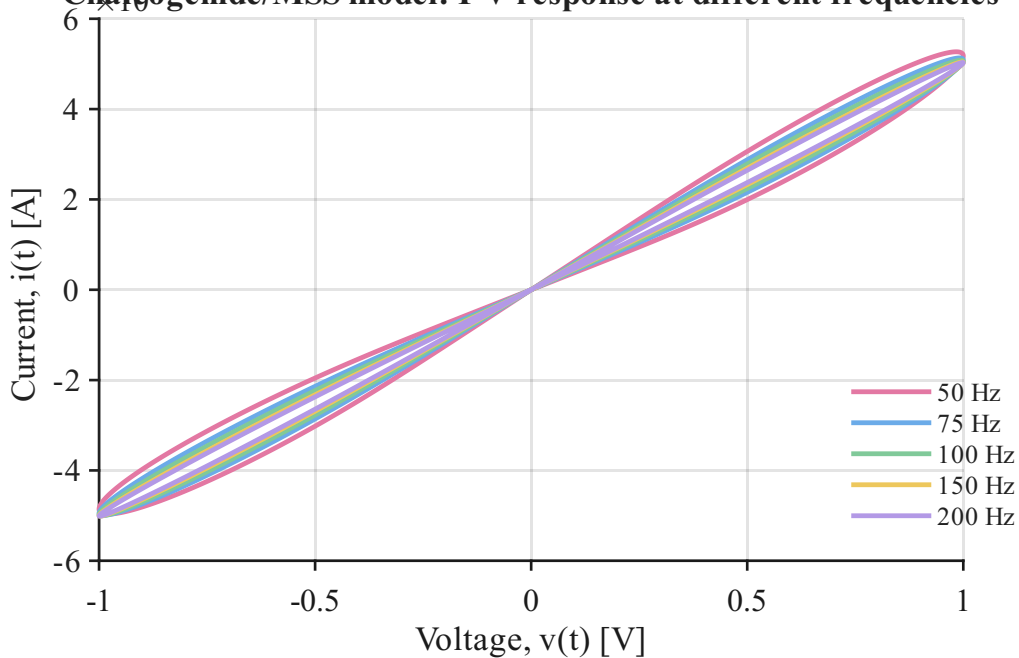
Chalcogenide/MSS model: I-V response at different frequencies
