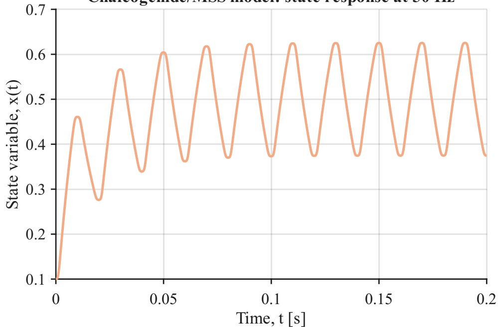
Chalcogenide/MSS model: state response at 50 Hz
