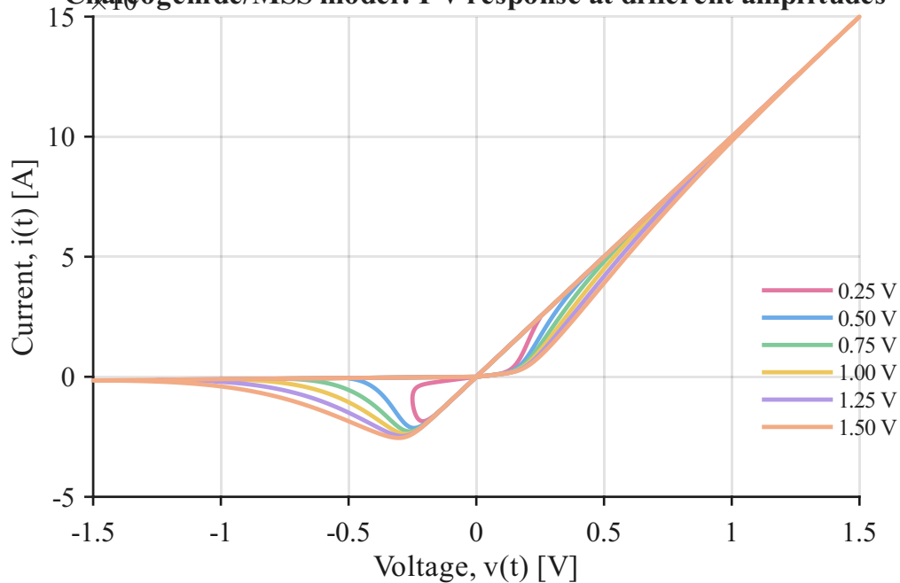
Chalcogenide/MSS model: I-V response at different amplitudes
