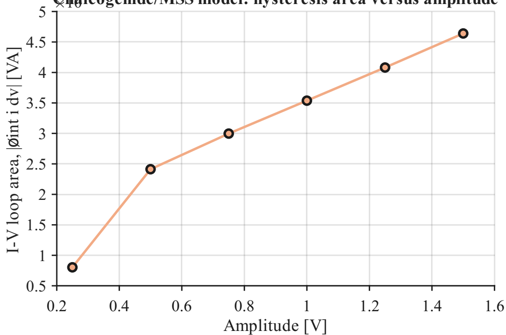
Chalcogenide/MSS model: hysteresis area versus amplitude
