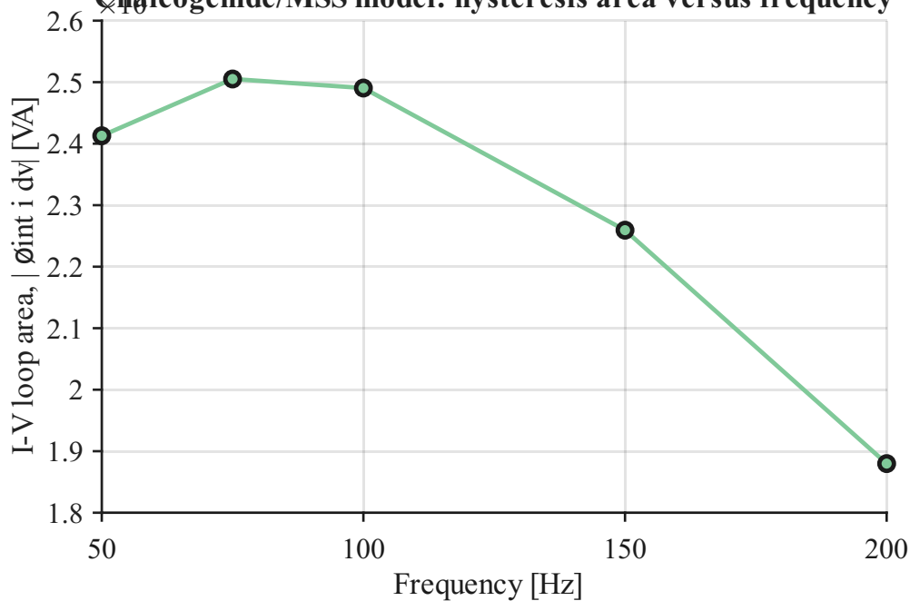
Chalcogenide/MSS model: hysteresis area versus frequency
