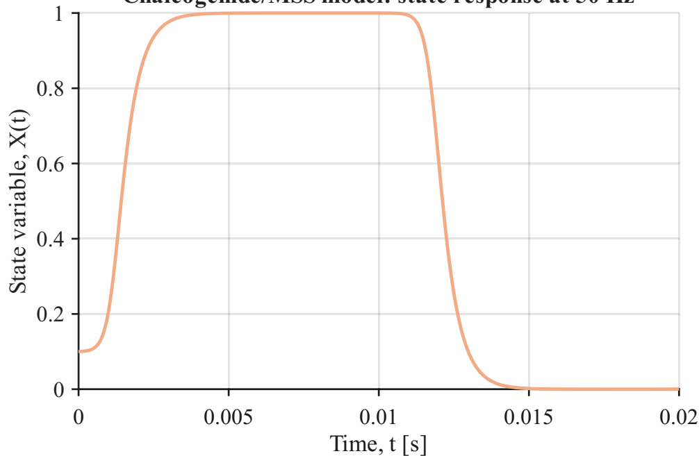
Chalcogenide/MSS model: state response at 50 Hz
