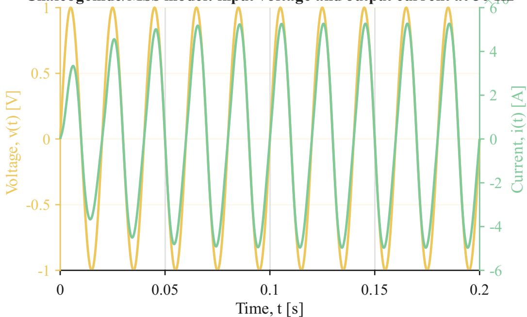
Chalcogenide/MSS model: input voltage and output current at 50 Hz 3
