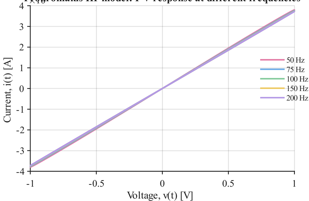
Prodromakis HP model: I-V response at different frequencies
