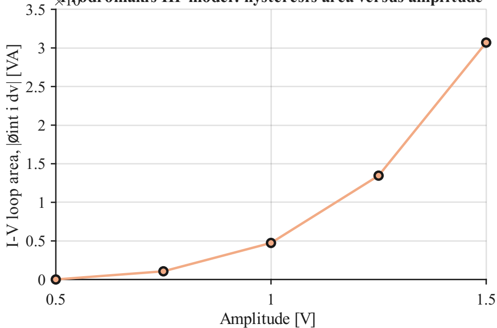
Prodromakis HP model: hysteresis area versus amplitude
