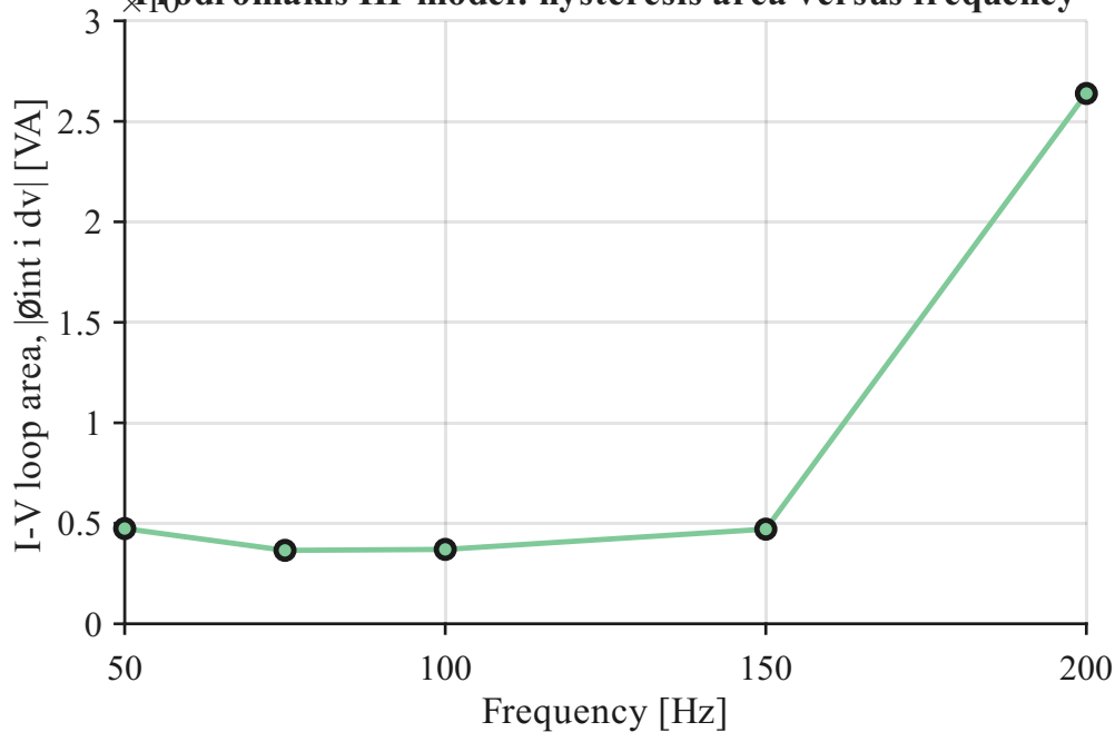
Prodromakis HP model: hysteresis area versus frequency
